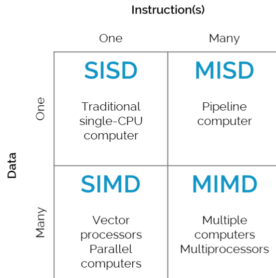
Figure 1 - Flynn's Taxonomy
